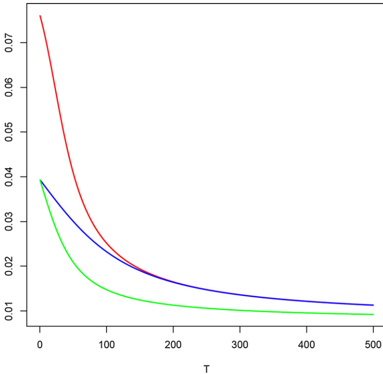
Fig. 3. This figure represents the socially efficient discount rate for \gamma_1 = \gamma_2 , \eta = 0.4 , \rho = 0 , \mu = 0.018 , \sigma = 0.036 , and \delta = 0.35 as well as the curves associated to the \eta -average (resp. arithmetic average) of the individual discount factors. The discount rate curve dominates the \eta -average that dominates the arithmetic average. With these parameters values, the rational rate is equal to 3.2%.
